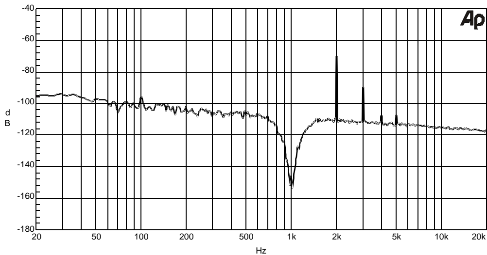
Graph 3: Noise spectrum
